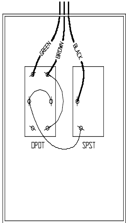
BOTTOM VIEW-COVER
